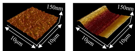
(a) SUJ2+a-C:H/Xylitol Solution (b) SUJ2/Gear oil
