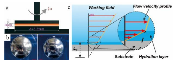
Fig.1 Construction of thermodynamic solid-liquid interface and the characterization of coupling effect.
