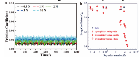
Fig.2 Super-hydrophilic surface with ultralow friction character and fluid drag reduction behavior.
